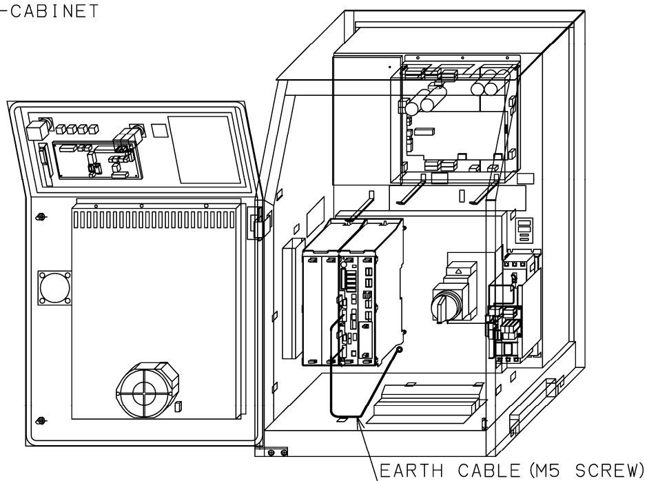
Fig. B.6(a) R-30iA earth cable
